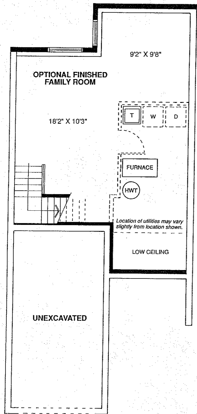
BASEMENT PLAN
