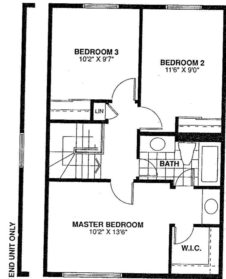
SECOND FLOOR AREA = 601 SQ. FT. TOTAL AREA = 1100 SQ. FT.
